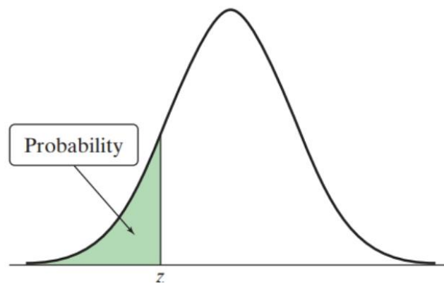
Standard Normal Probabilities [P(z ≤ 0)]
