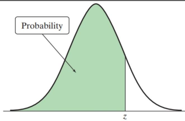
Standard Normal Probabilities [ P(z \geq 0) ]
